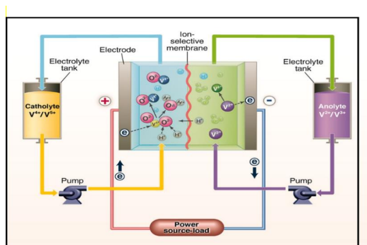
Fig. 1.5 Schematic representation of the vanadium redox flow battery as an example of redox flow batteries
