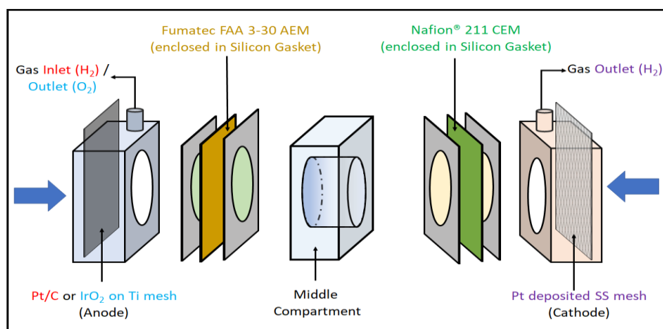
Fig 2.6 Diagrammatic representation of three-compartment cell assembly
